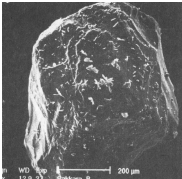
Fig. 2. Quartz grain weakly rounded, with secondary crystals on the surface.
