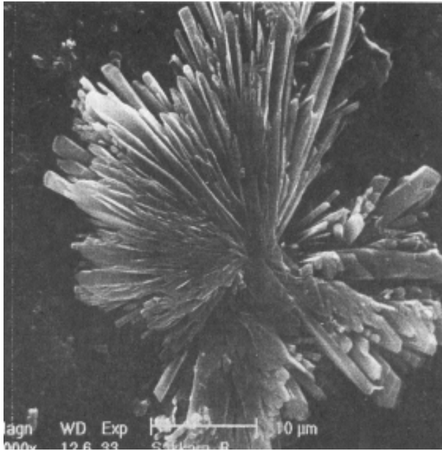
Fig. 4. Gypsum aggregate crystallized on quartz grain surface.
