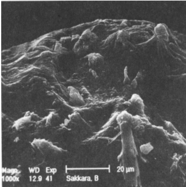
Fig. 5. Fragment of quartz grain surface with secondary minerals (probably ardealite).
