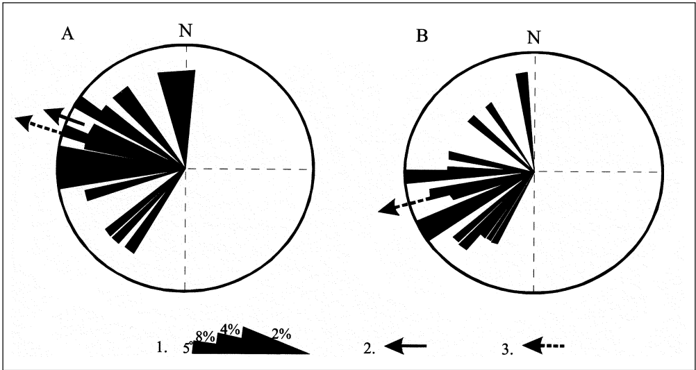
Fig. 6. Distribution of the longer axis orientation in pebbles 0/5-9.5 cm fraction, from the upper level of the site (Shaft 16, Figs 1,4) presented as a circle diagram: A - NW part of the downhill flow; B - SW part of the downhill flow; 1 -percentage share of pebbles in 5 \circ angle sectors; 2 - direction of downhill water flow estimated on the basis of inclination of sandy layers; 3 - average vector of downhill water flow direction estimated on the basis of longer-axis orientation of pebbles
