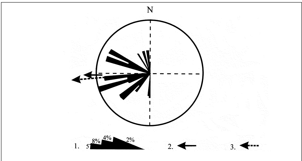
Fig. 7. Distribution of the longer axis orientation in pebbles of 5.5-11 cm fraction from the section in line with Shaft 1 [Figs. 1, 5]: 1 - percentage share of pebbles in 5 \circ angle sectors; 2 - direction of downhill water flow estimated on the basis of inclination of sandy-gravel layers; 3 - average vector of downhill water flow direction estimated on the basis of longer axis orientation of pebbles
