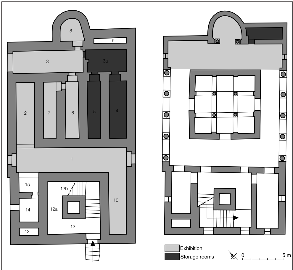
Fig. 15. The Mosque, concept of interior adaptation, ground floor and first floor (Design W. Kolątaj, S. Medeksza)
